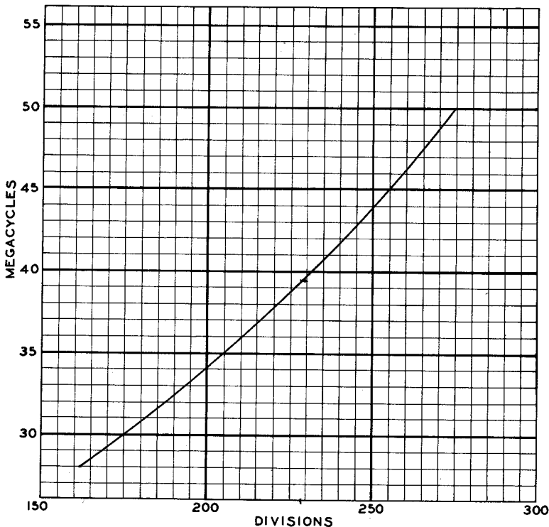
CALIBRATION OF COIL H 605-A STANDARD SIGNAL GENERATOR SERIAL # 442
