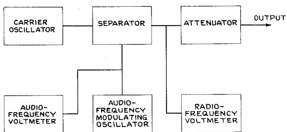
Figure 5. Functional Diagram of Type 605-A Standard-Signal Generator
